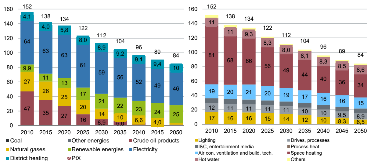
Figure 13: Development of energy consumption of services by energy source (left) and type of use (right) in PJ according to the ZERO basis scenario of EP2050+. Source: Prognos/TEP Energy/Infras/Ecoplan 2020, unpublished detailed data.
