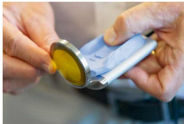
Elastic membrane, olive oil as a coupling fluid: Veinpress pressure gauge for measuring central venous pressure.
