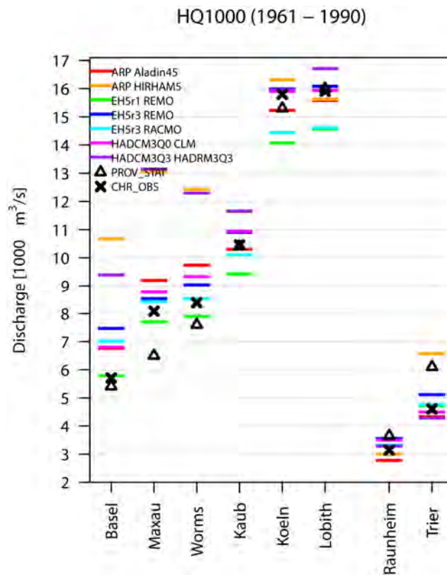
Figure 3-27: As in Figure 3-24, but HQ1000 [ \text{m}^3/\text{s} ]. Except for the observed PROV_STAT the results are based on the 3000-year re-sampled timeseries.
