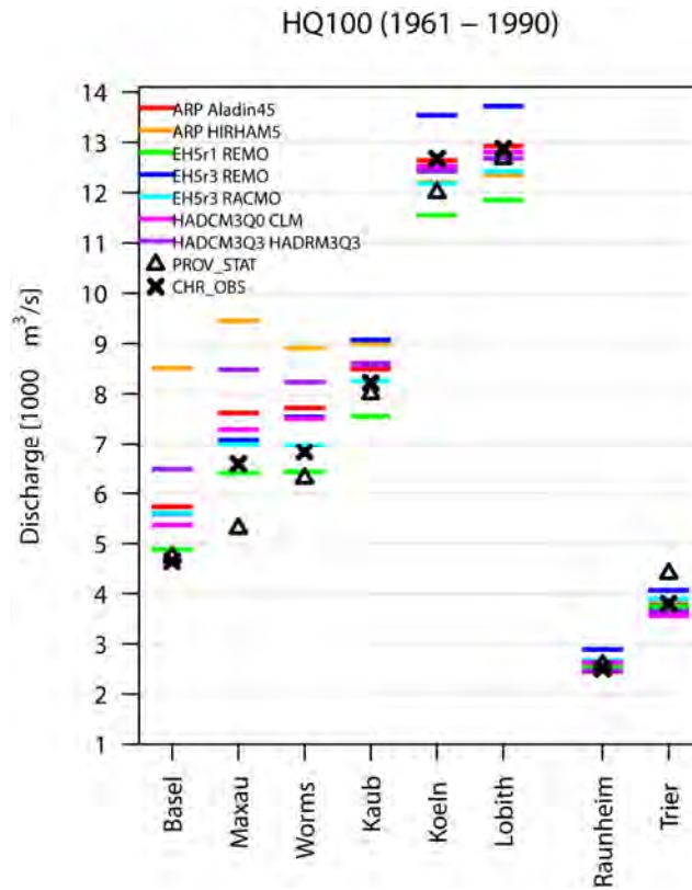
Figure 3-26: As in Figure 3-24, but HQ100 [ \text{m}^3/\text{s} ]. Except for the observed PROV_STAT the results are based on the 3000-year re-sampled timeseries.
