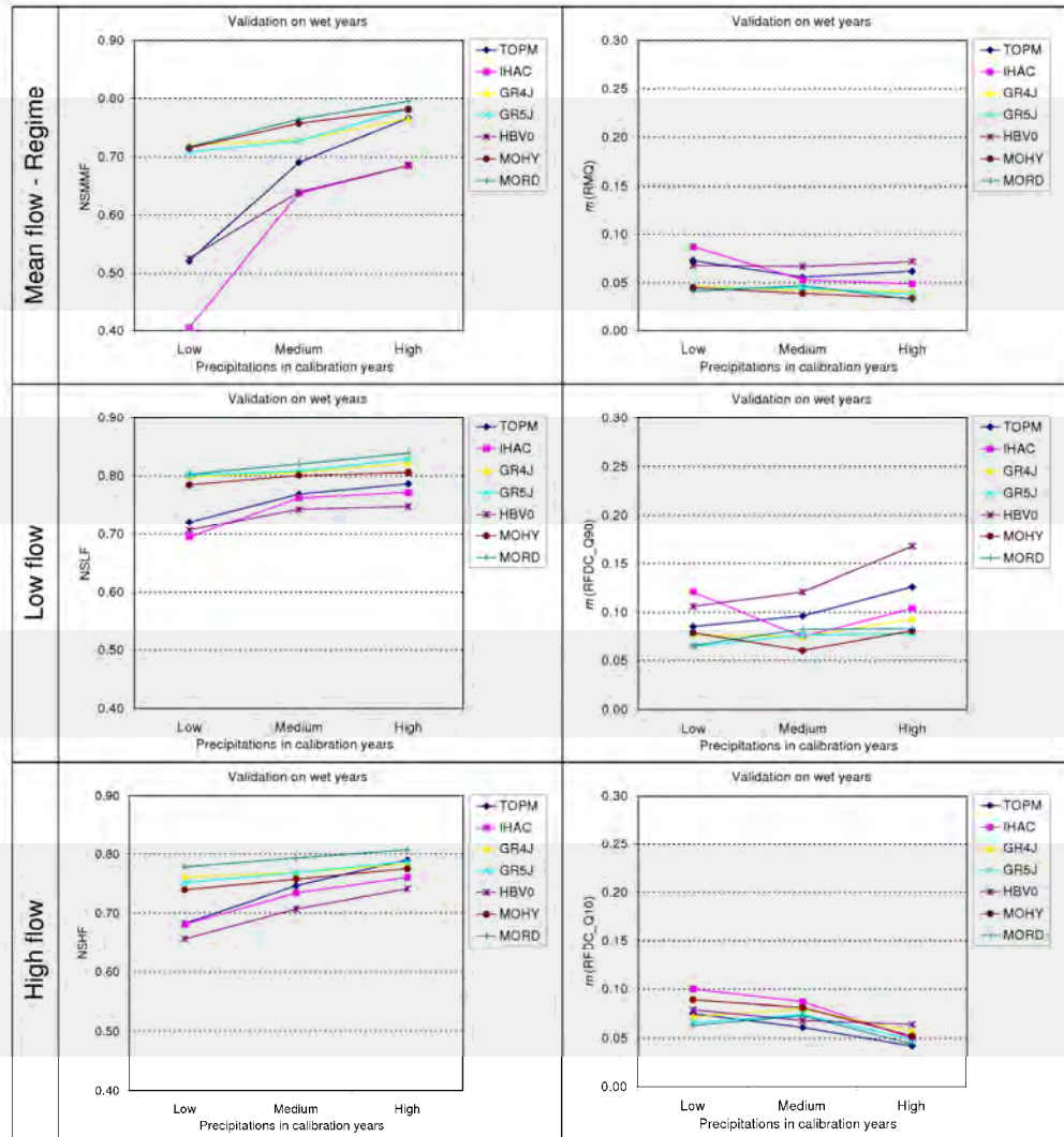
Figure D-1: Sensitivity of model results to the calibration conditions: case of model validation for wet years.
